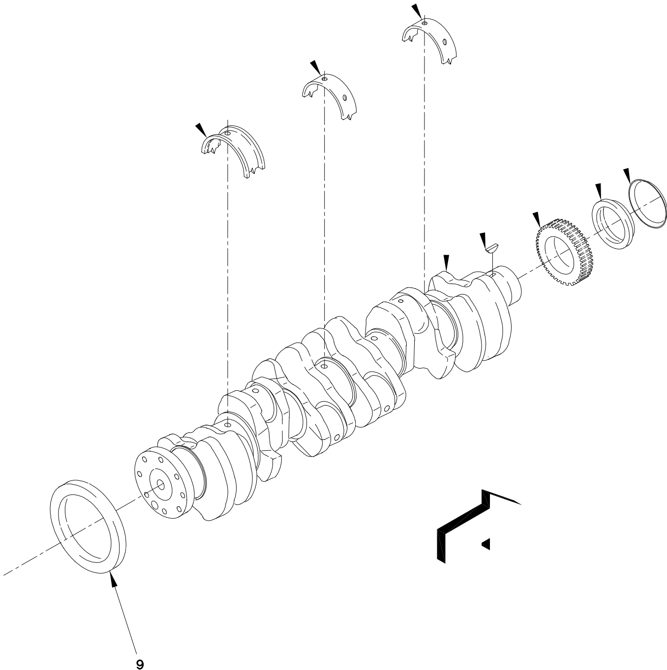
FIGURE 6. CRANKSHAFT
