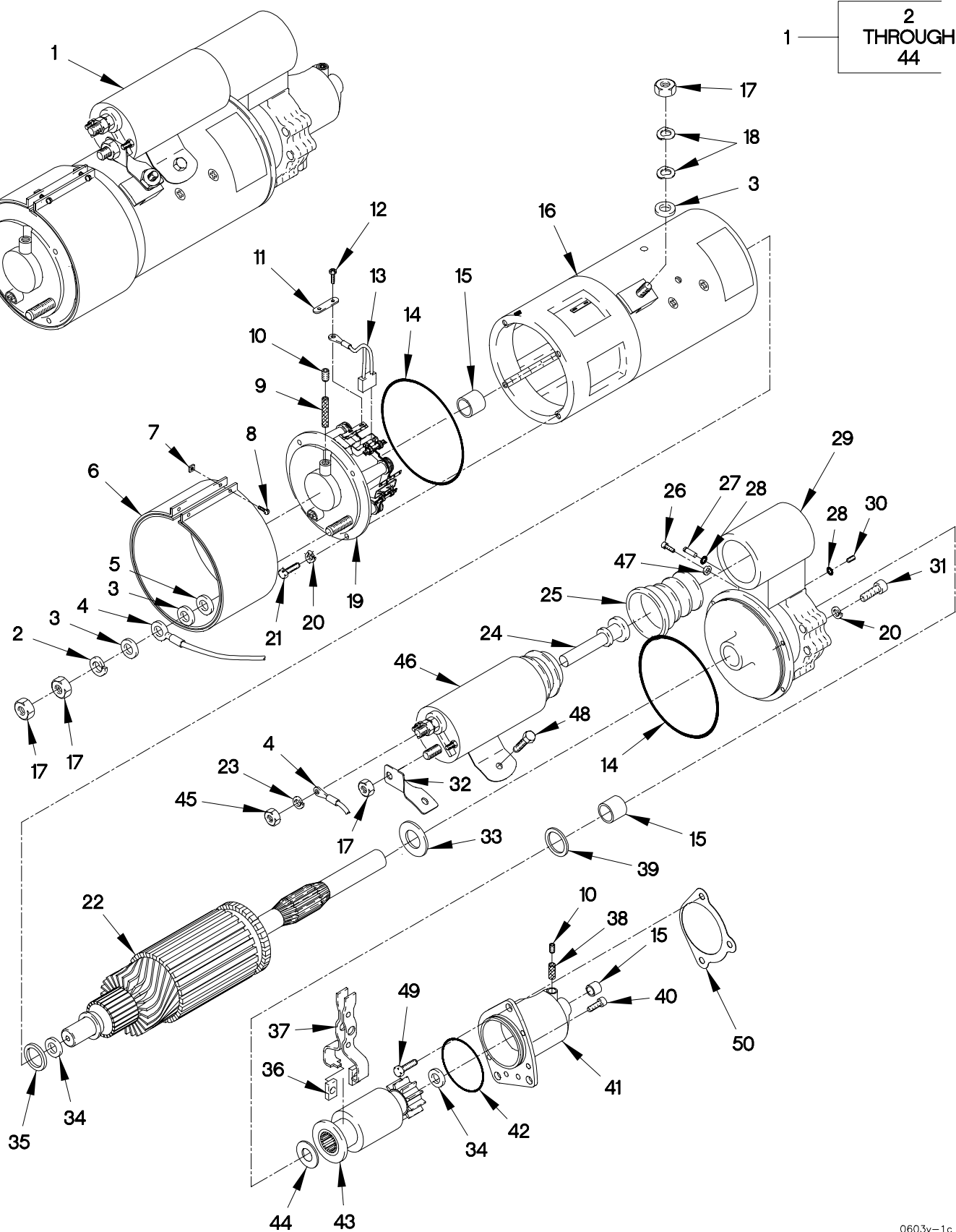
FIGURE 48. M0017703MD STARTER AND SOLENOID
