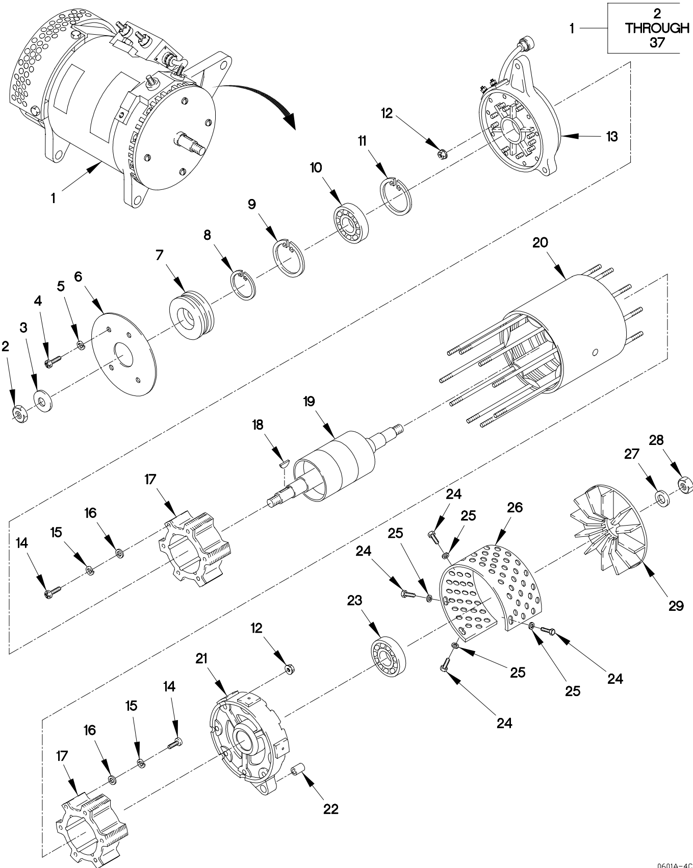
FIGURE 46. 100 AMP ALTERNATOR, BRACKETS AND BELT (SHEET 1 OF 2)
