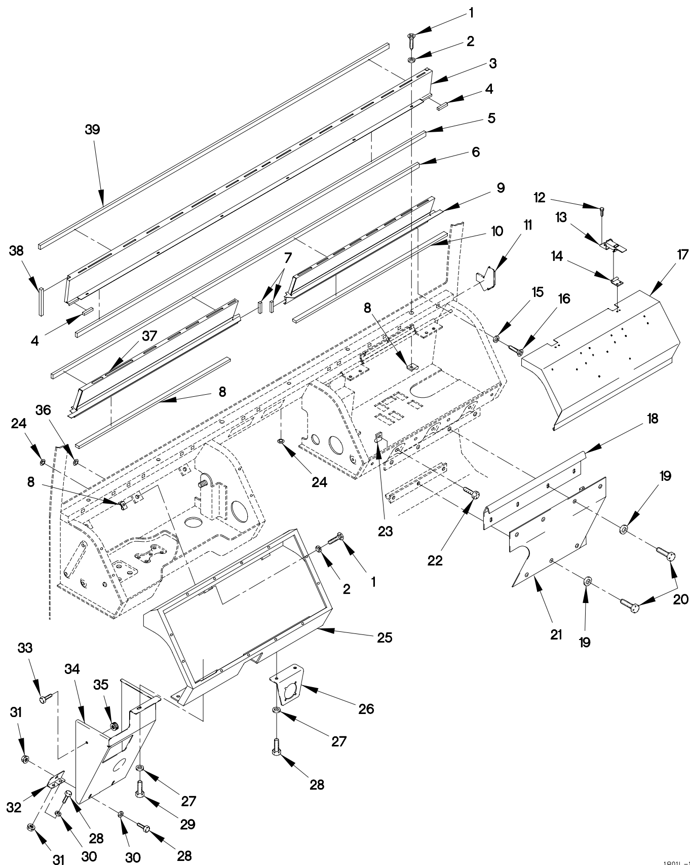
FIGURE 185. DASHBOARD
