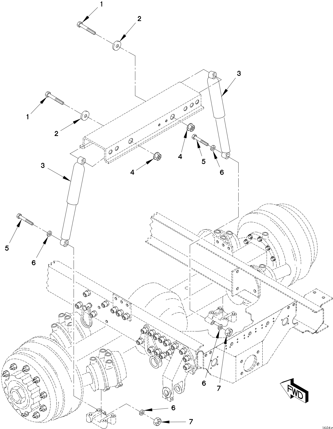
FIGURE 181. REAR SHOCKS
