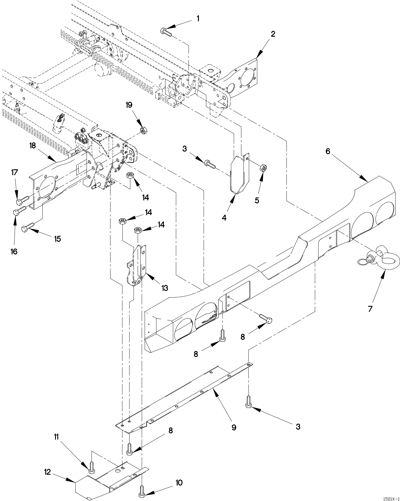
FIGURE 172. FRONT BUMPER AND GRAVEL DEFLECTOR
