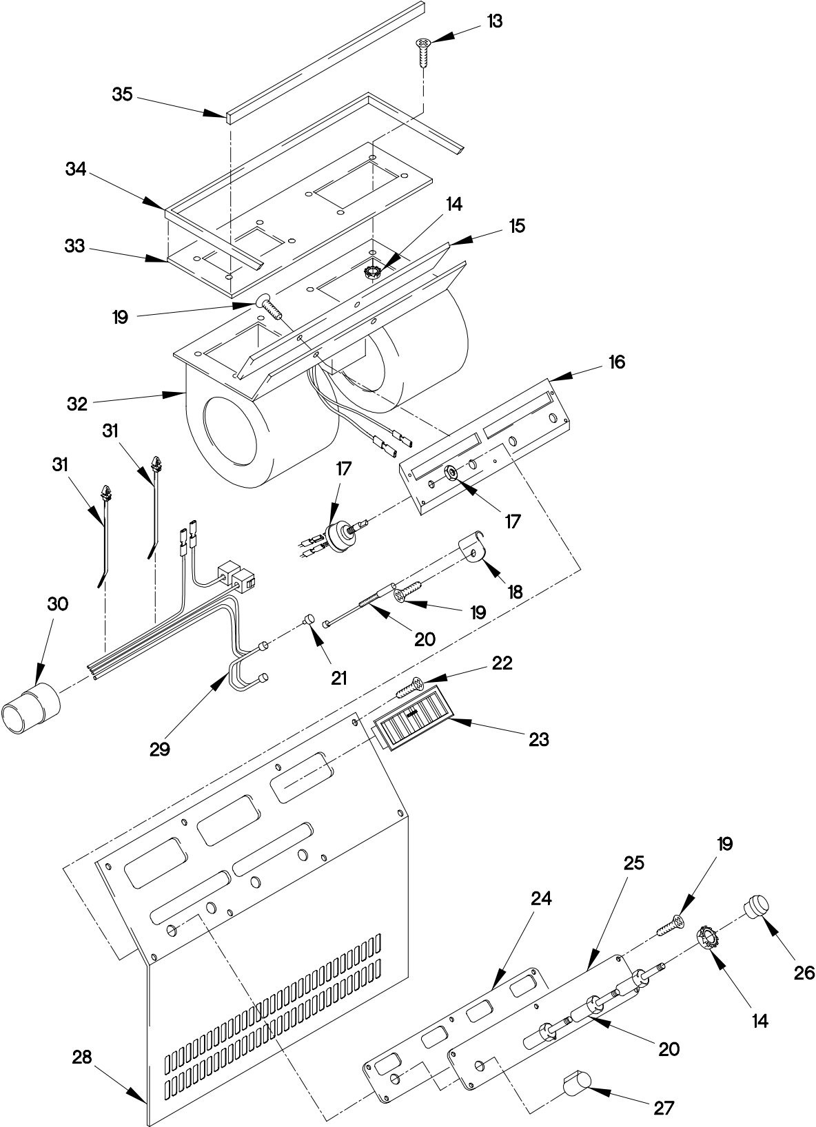
FIGURE 249. PERSONNEL HEATER ASSEMBLY (SHEET 2 OF 3)
