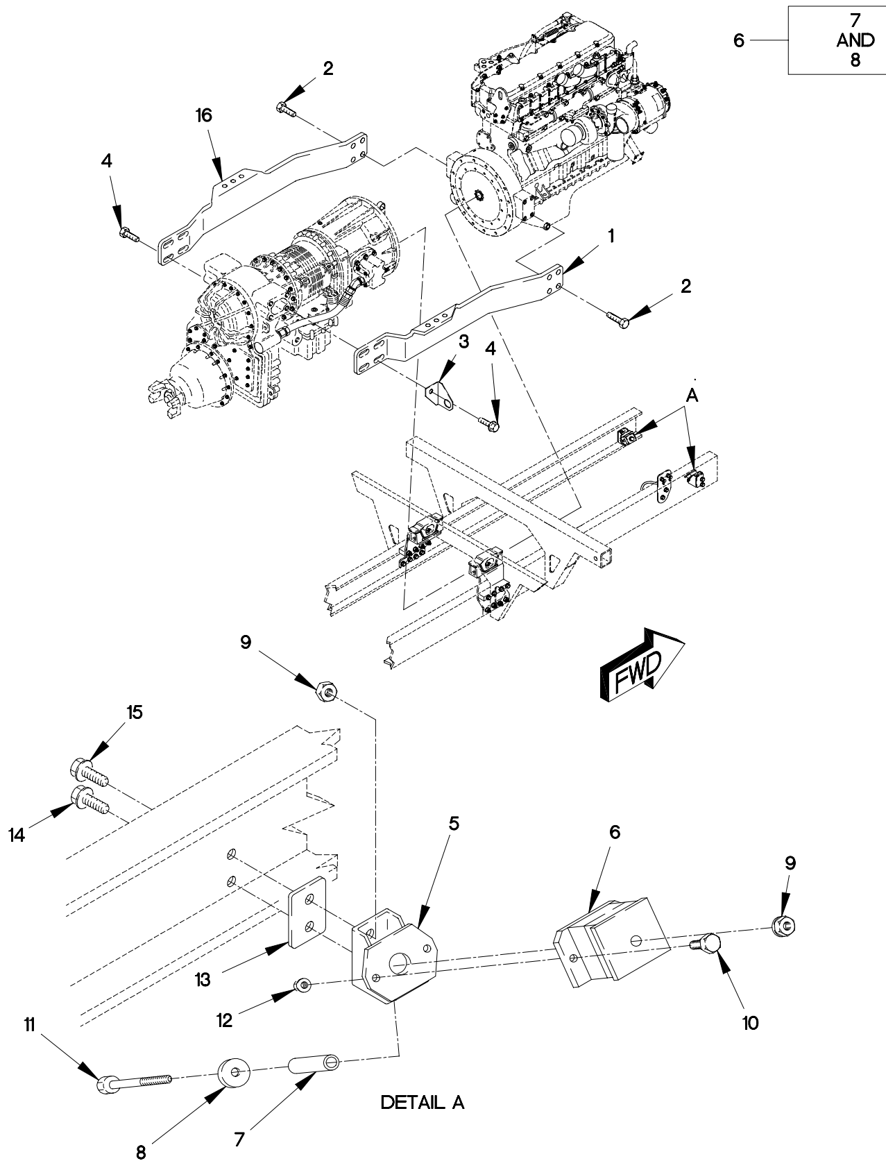
FIGURE 2. ENGINE MOUNTS
