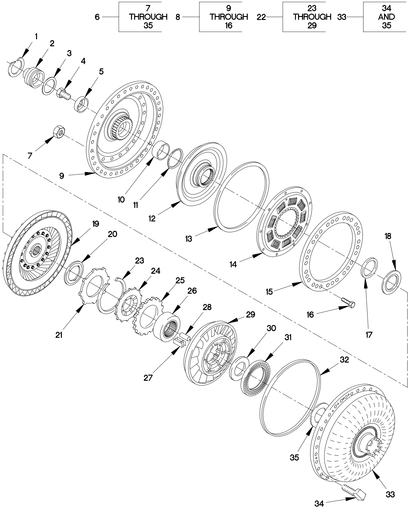
FIGURE 112. TORQUE CONVERTER MODULE
