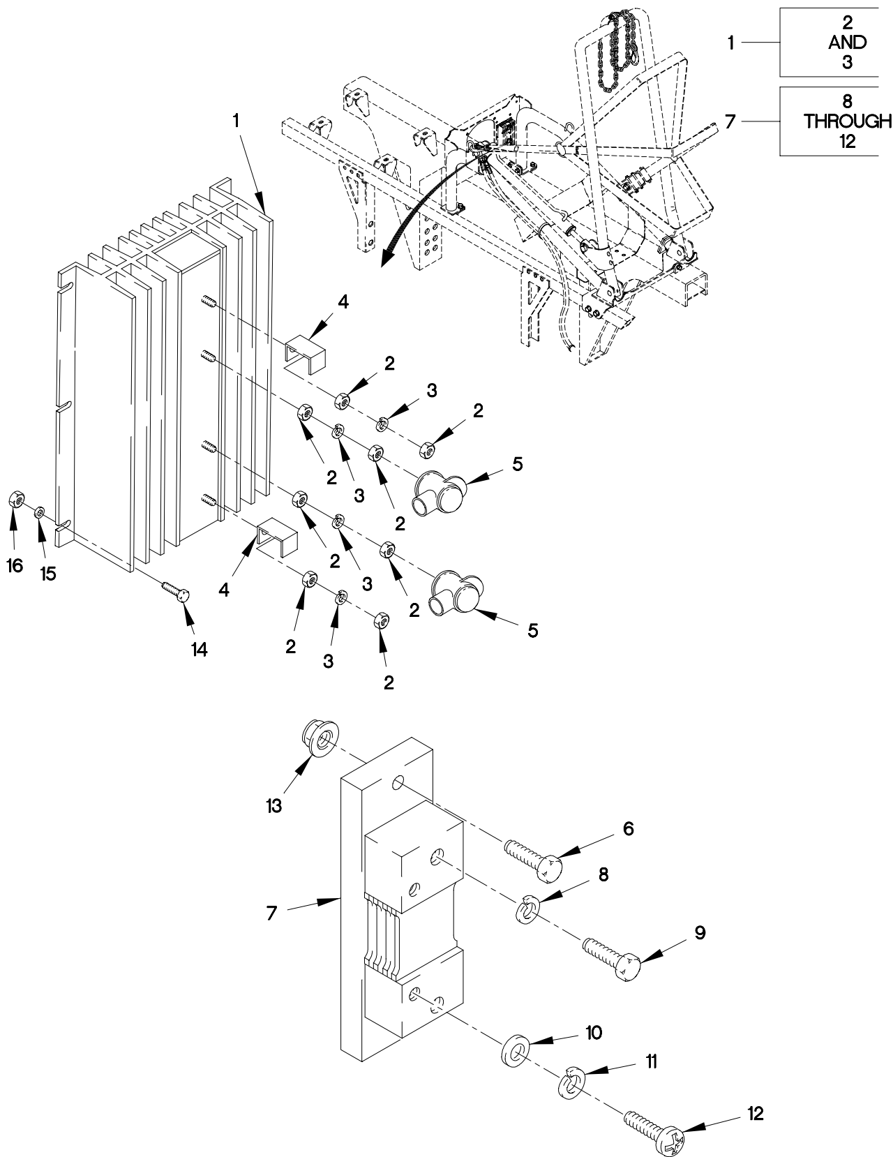
FIGURE 60. 100A REVERSE POLARITY RELAY AND STARTER SHUNT
