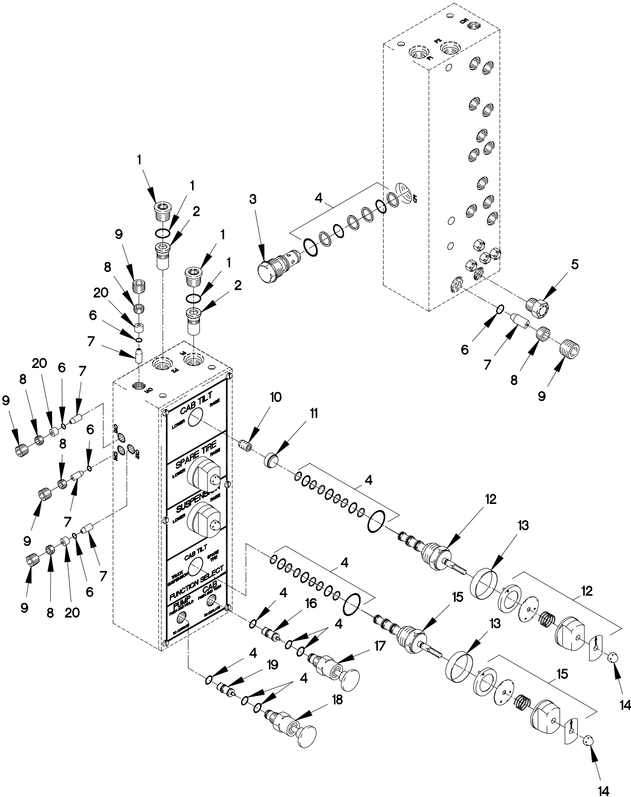
FIGURE 254. HYDRAULIC MANIFOLD ASSEMBLY
