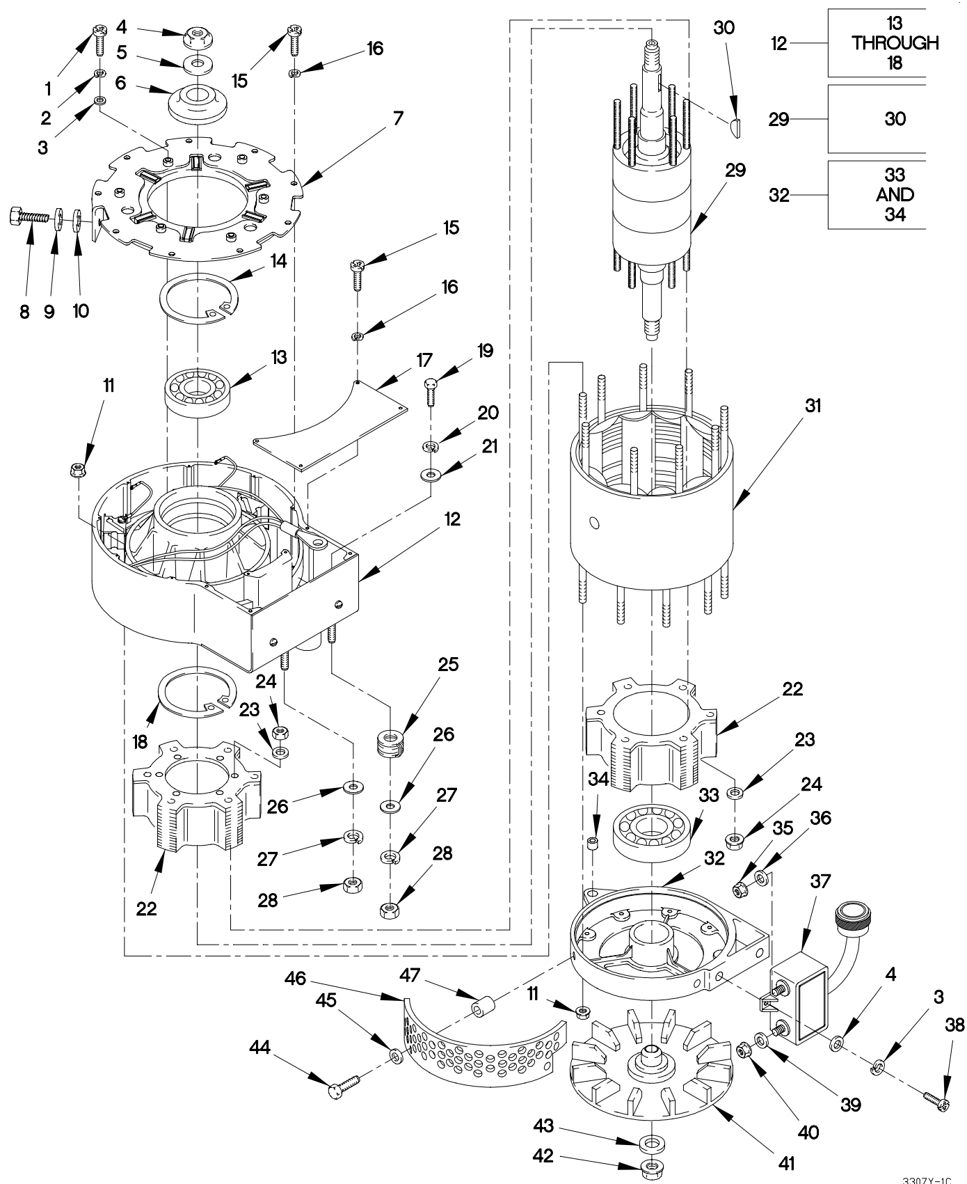
FIGURE 272. 200A ALTERNATOR AND REGULATOR
