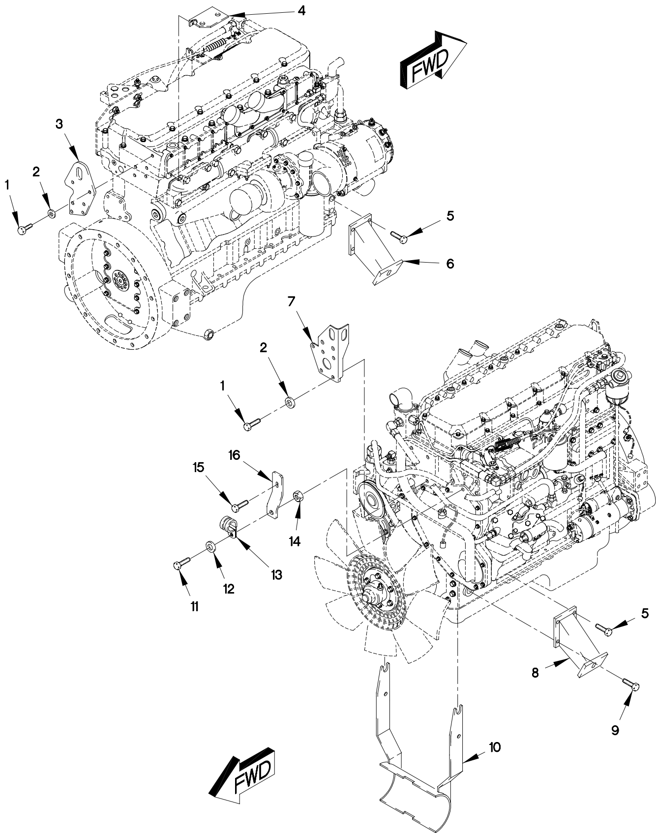
FIGURE 3. ENGINE BRACKETS
