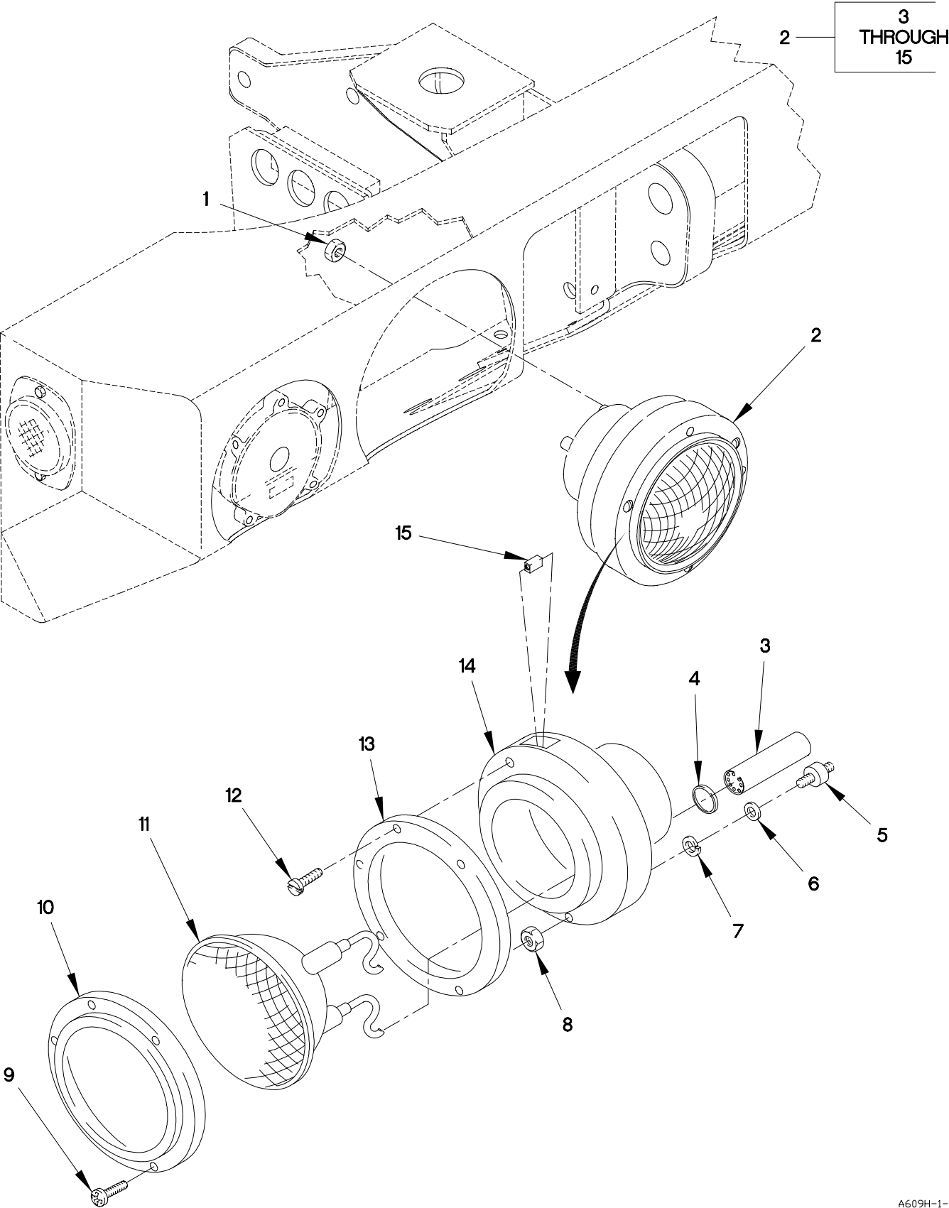
FIGURE 61. HEADLAMP ASSEMBLY
