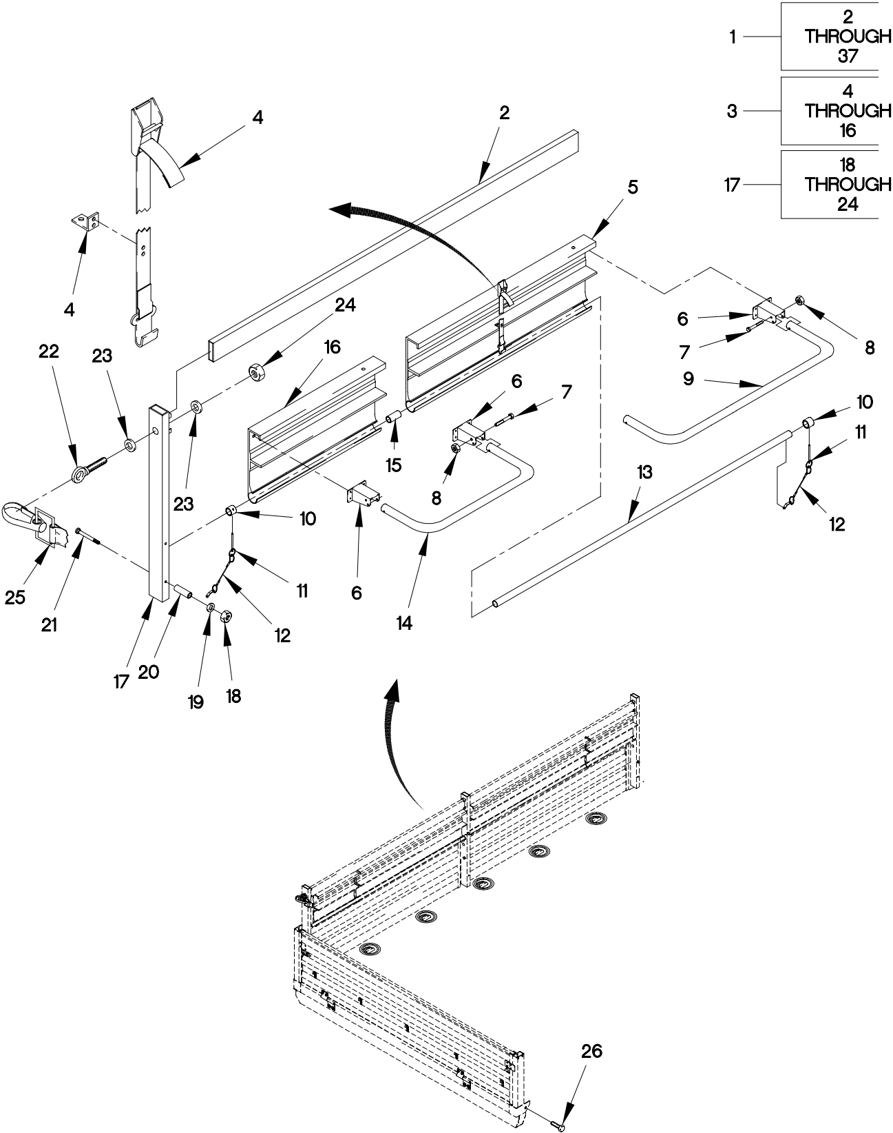
FIGURE 267. M1078 AND M1081 TROOPSEAT KIT (SHEET 1 OF 2)
