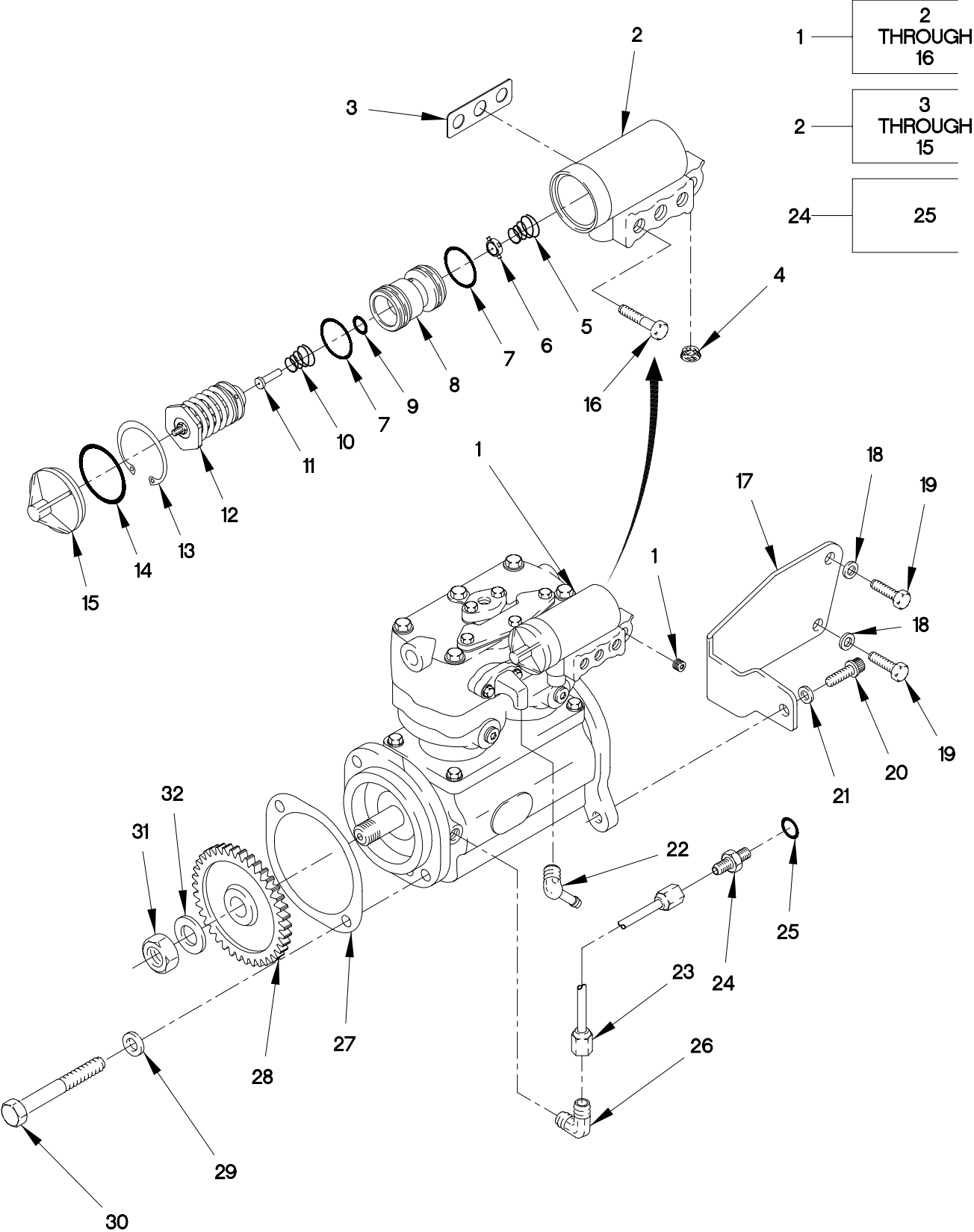
FIGURE 157. AIR COMPRESSOR
