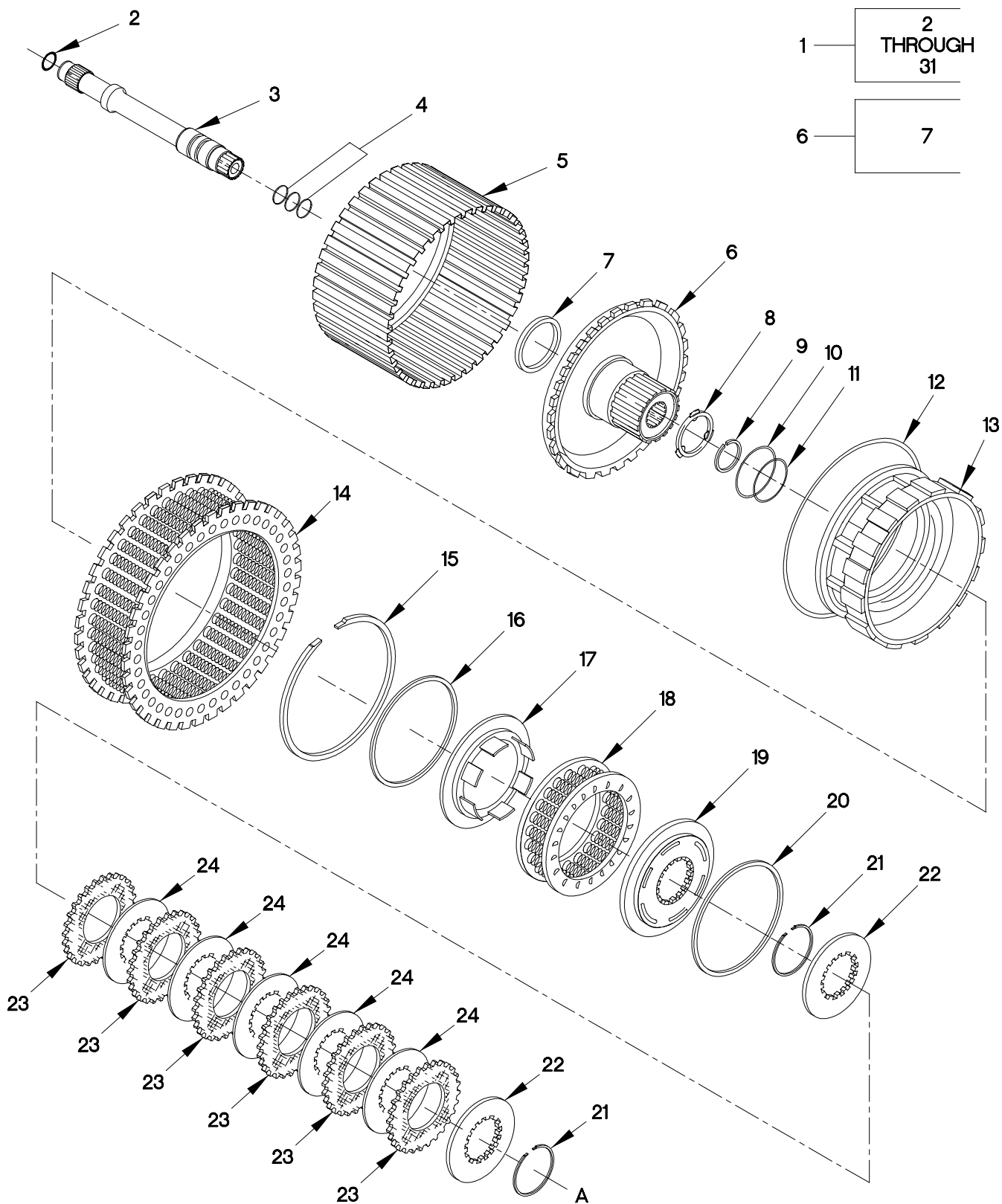
FIGURE 124. ROTATING CLUTCH MODULE (SHEET 1 OF 2)
