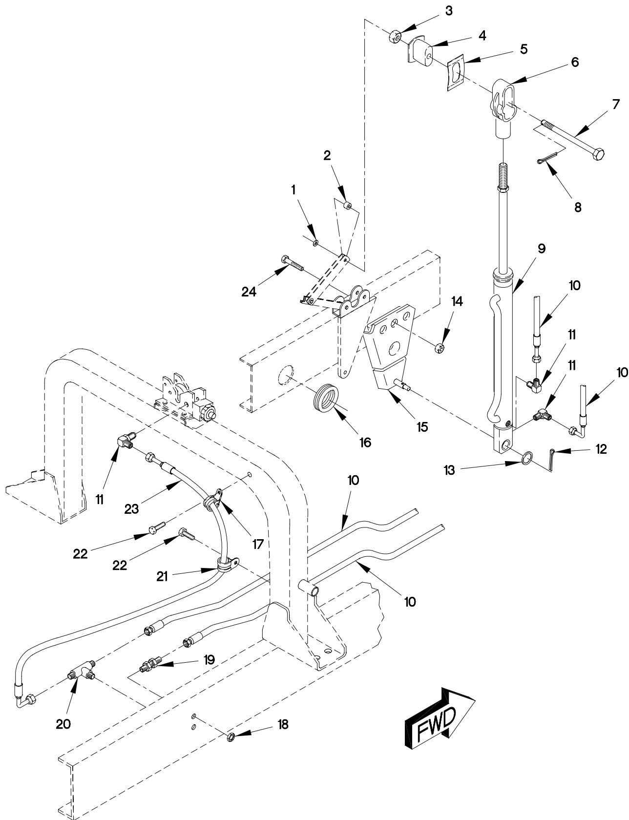
FIGURE 257. CAB HYDRAULIC CYLINDER, HOSES AND FITTINGS
