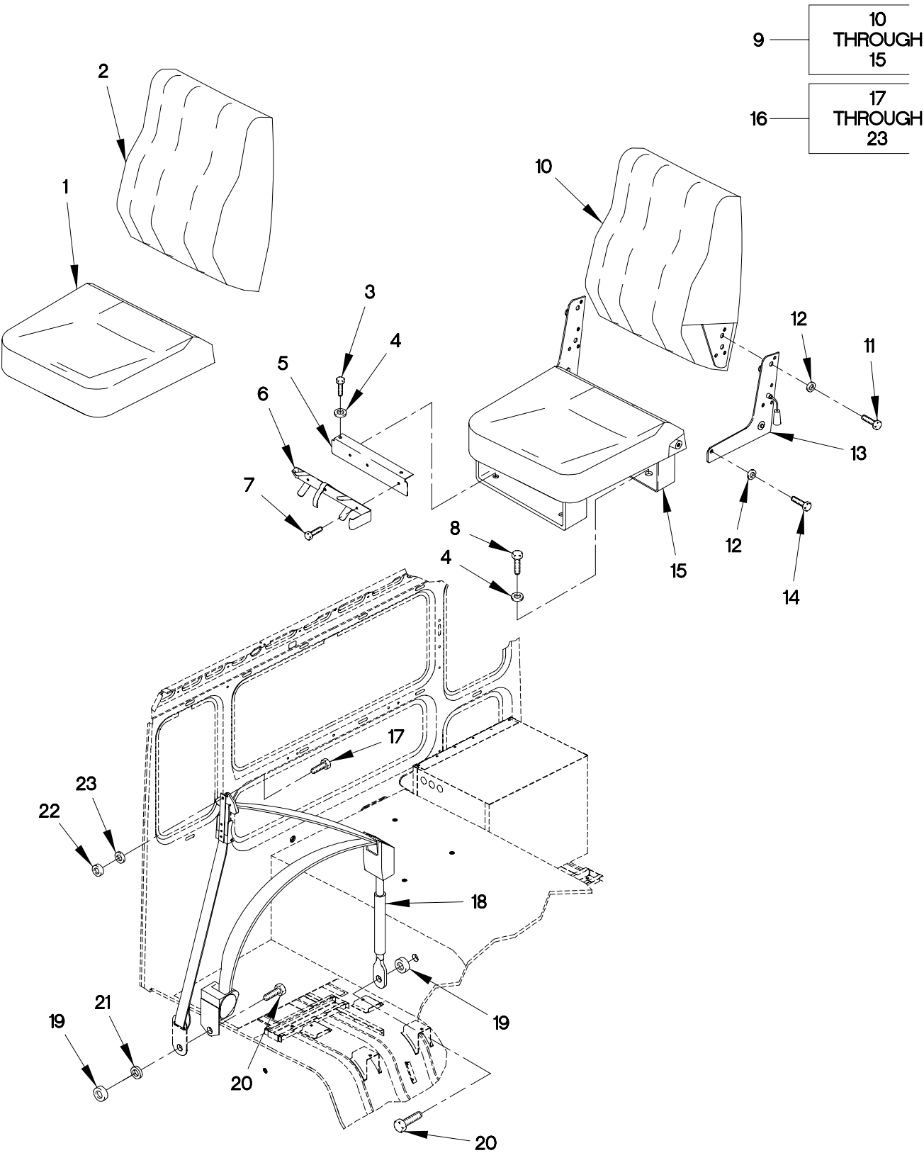
FIGURE 205. PASSENGER SEAT AND SEAT BELT
