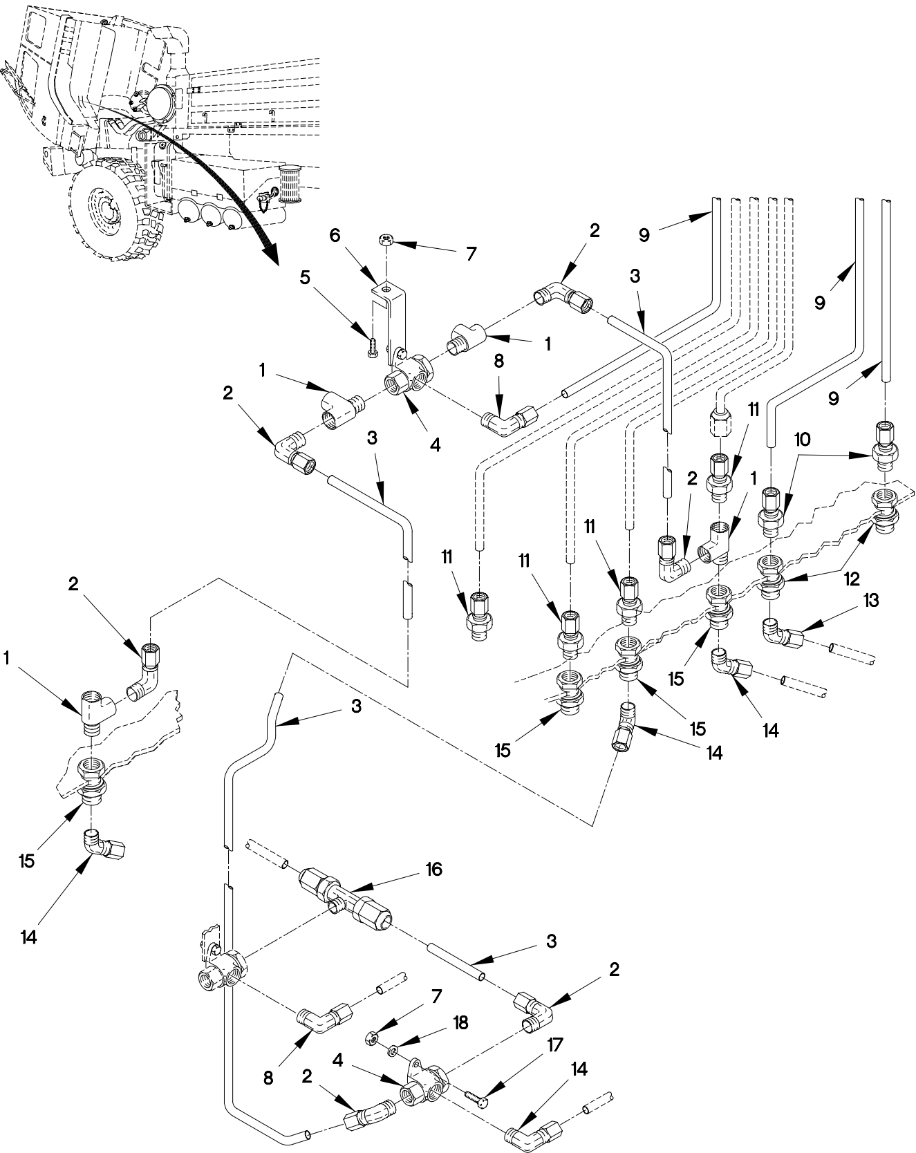
FIGURE 155. PARK CONTROL, EMERGENCY/SERVICE TWO WAY CHECK VALVE, HOSES AND FITTINGS
