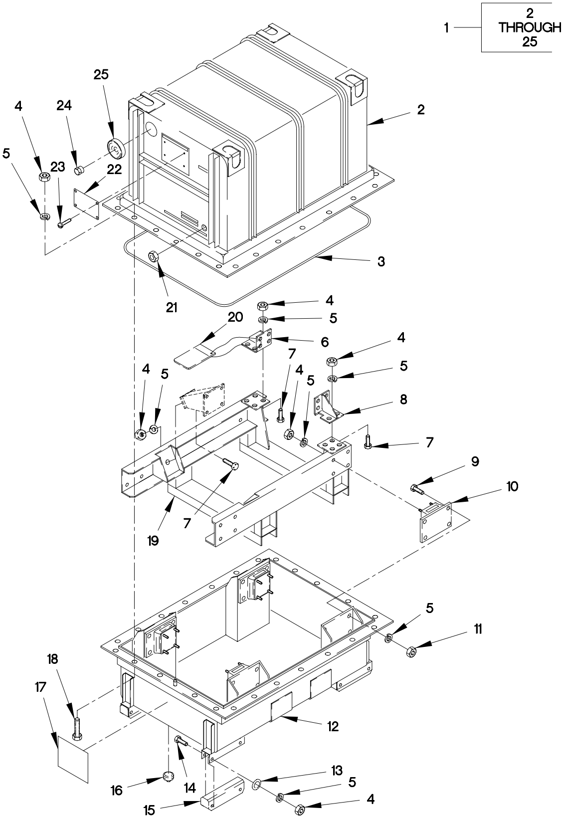
FIGURE 261. ENGINE CONTAINER
