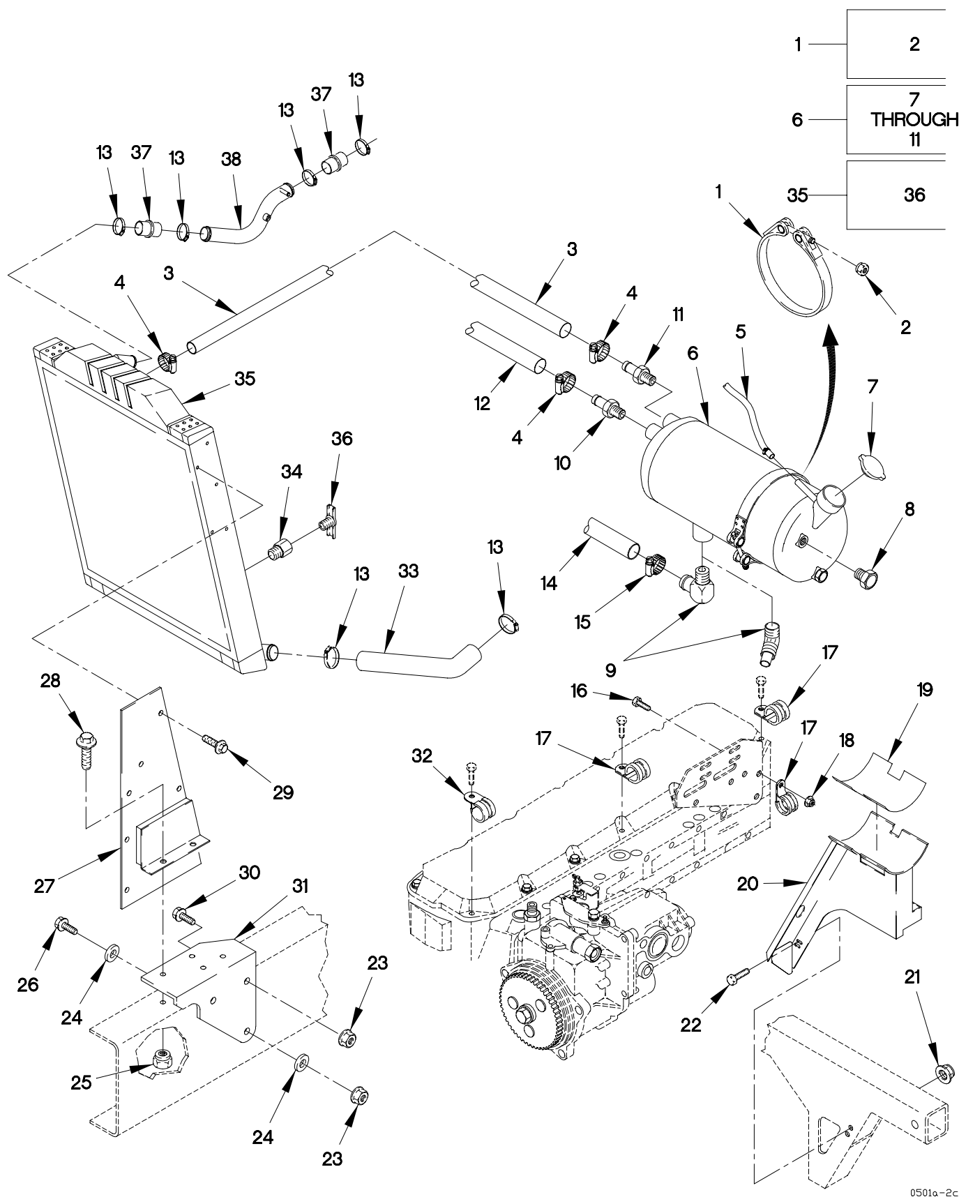
FIGURE 41. RADIATOR, OVERFLOW TANK, HOSES AND FITTINGS
