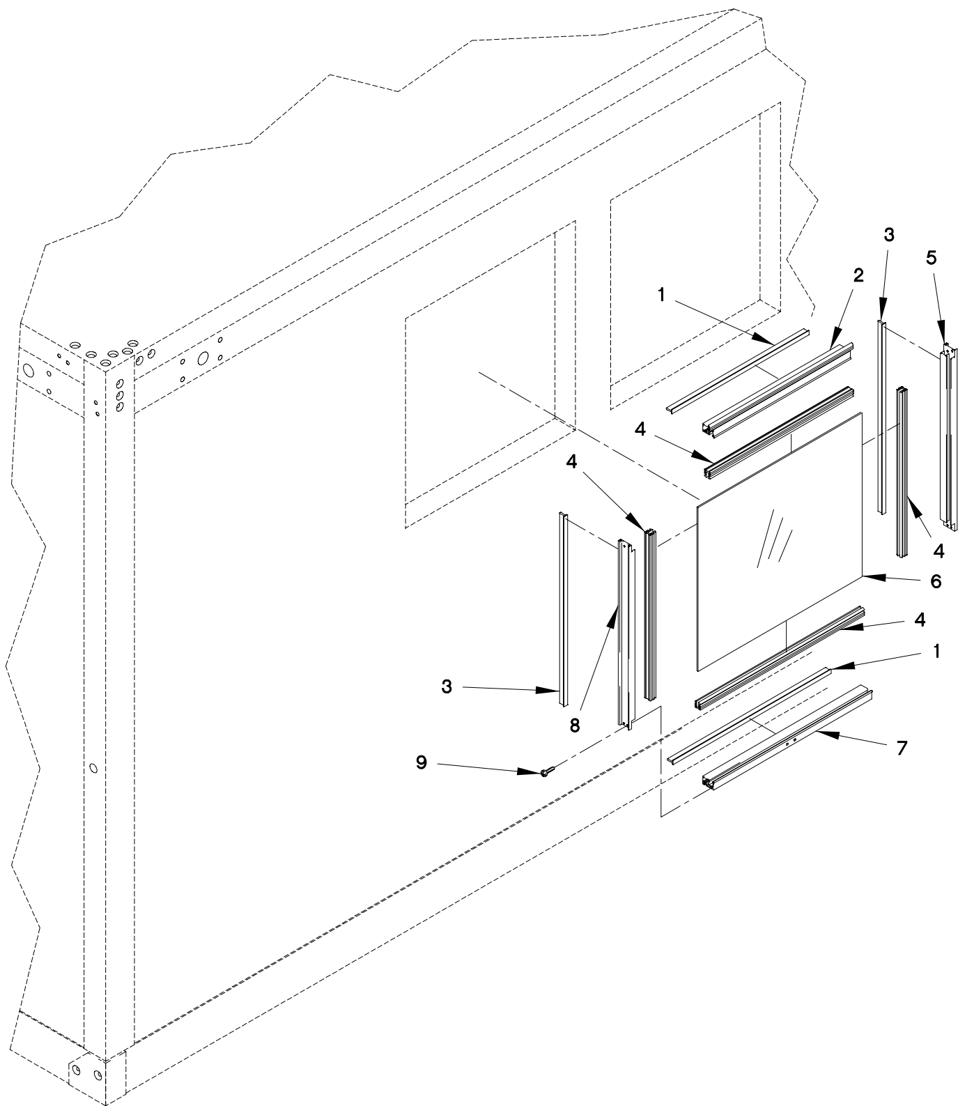
FIGURE 226. VAN LARGE WINDOW ASSEMBLY (SHEET 1 OF 3)
