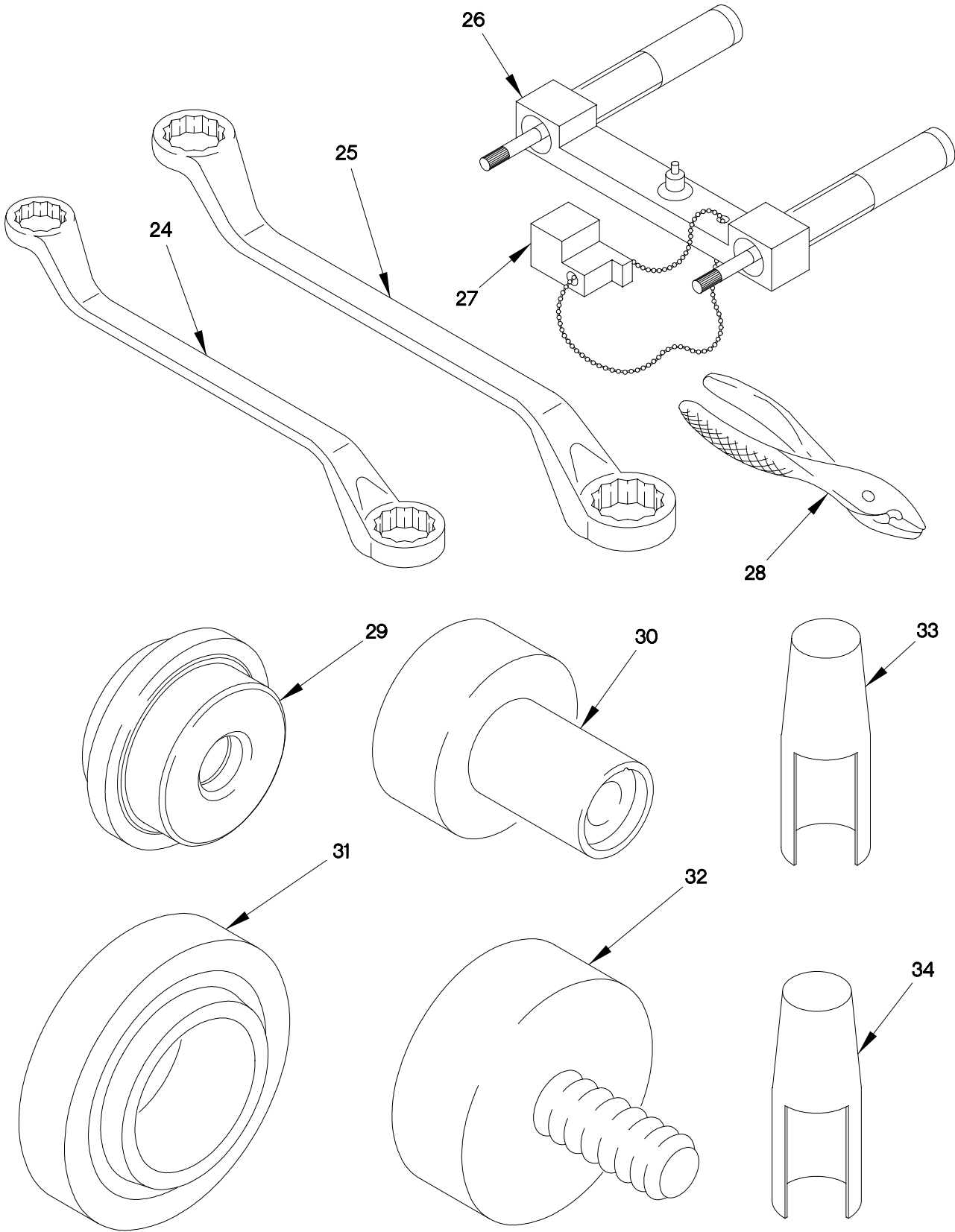
FIGURE 290. DIRECT SUPPORT MAINTENANCE SPECIAL TOOLS (SHEET 3 OF 3)
