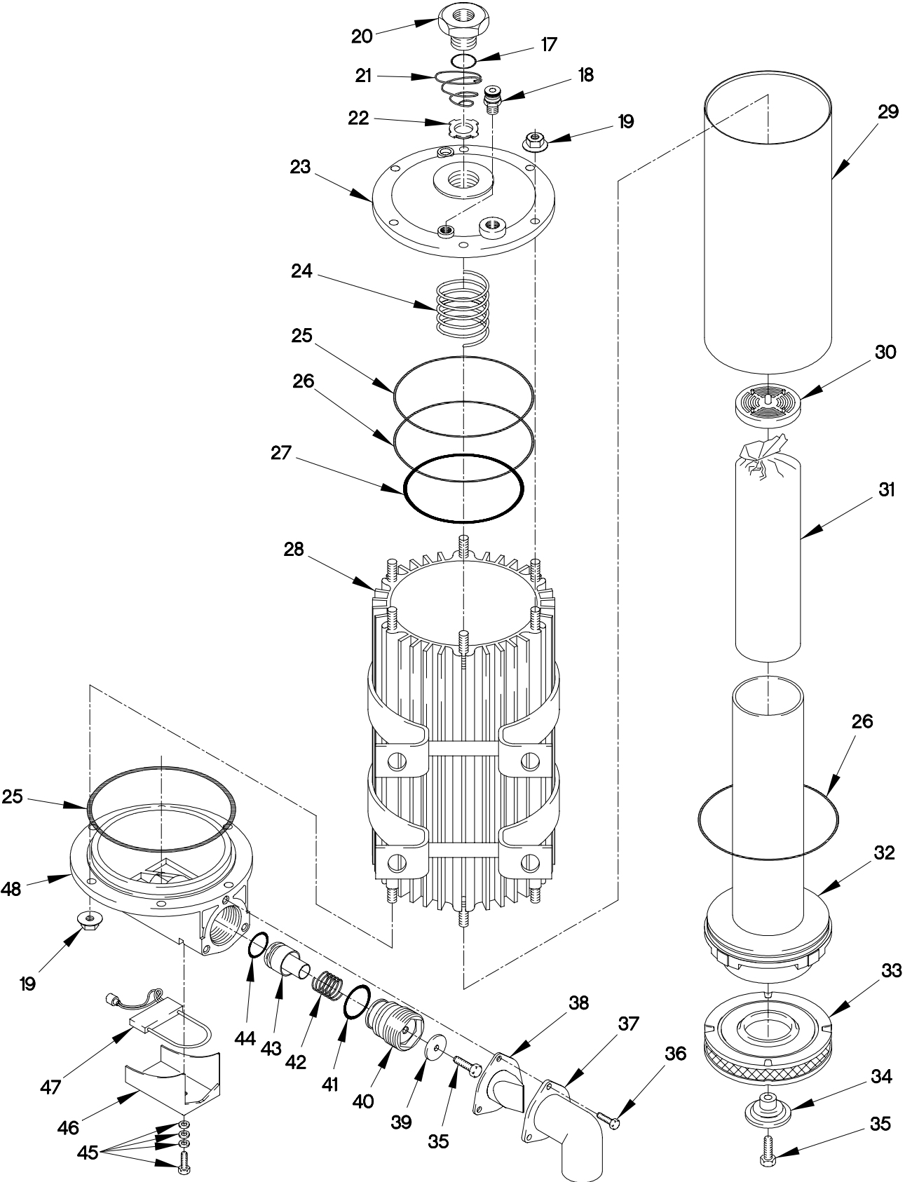
FIGURE 286. AIR DRYER, HOSES AND FITTINGS (SHEET 2 OF 2)
