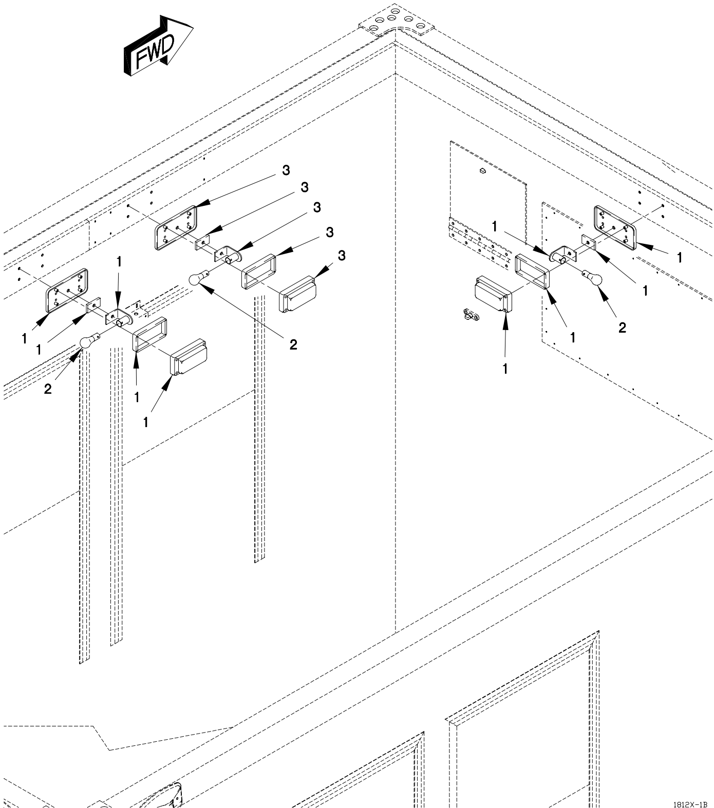
FIGURE 232. VAN BLACKOUT AND EMERGENCY LIGHTS
