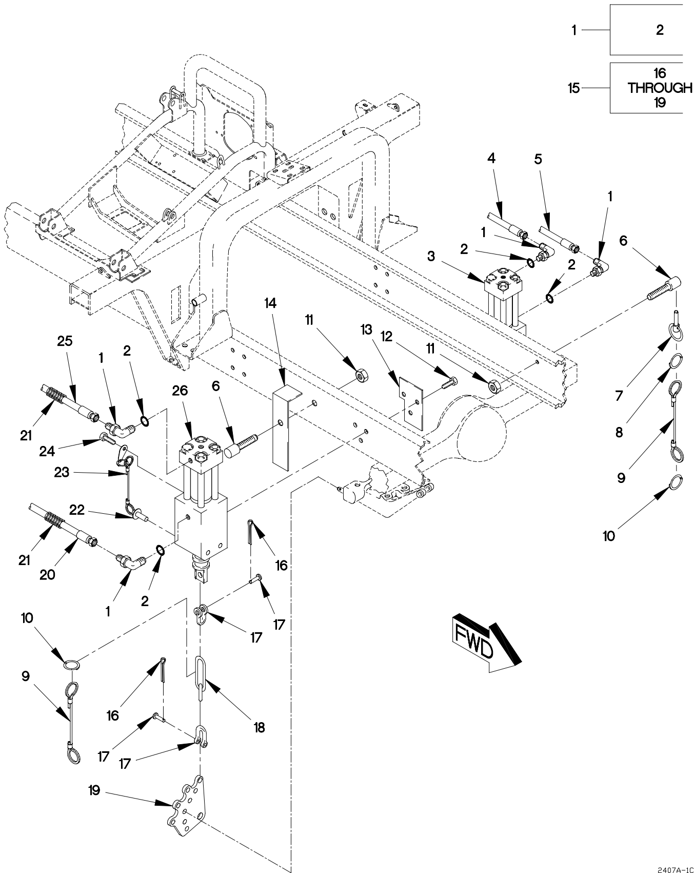
FIGURE 259. SUSPENSION CYLINDER HOSES AND FITTINGS
