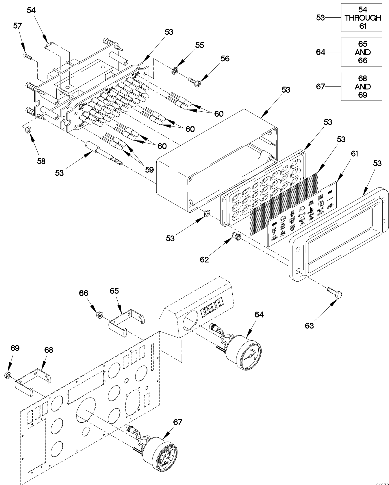
FIGURE 52. INSTRUMENT PANEL (SHEET 3 OF 3)
