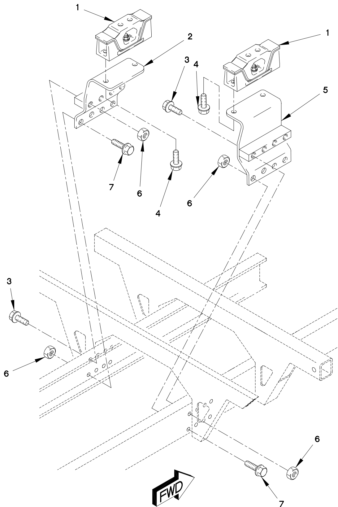
FIGURE 114. TRANSMISSION MOUNTS
